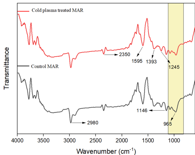
Fig. 2 FTIR spectra of untreated and cold plasma treated millet-based analogue rice.
